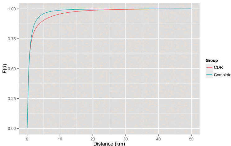
Figure 9. Cumulative distribution function (CDF) of displacements.
