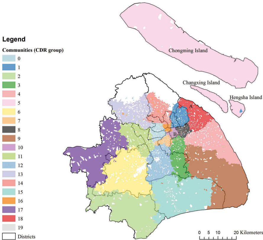
Figure 11. Detected communities based on the CDR group.
