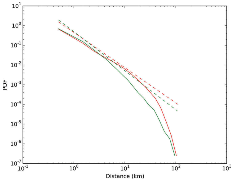
Figure 10. Probability density function (PDF) and the fitted power law distribution. The green line and red line represent the probability distribution of the displacements derived from the CDR group and the complete group, respectively. The dashed green line and the dashed red line are the fitted power law distributions for the CDR group and the complete group, with a decay parameter of 1.79 and 1.98, respectively.
