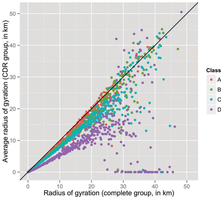
Figure 7. Radius of gyration (complete group) vs. average radius of gyration (CDR group).
