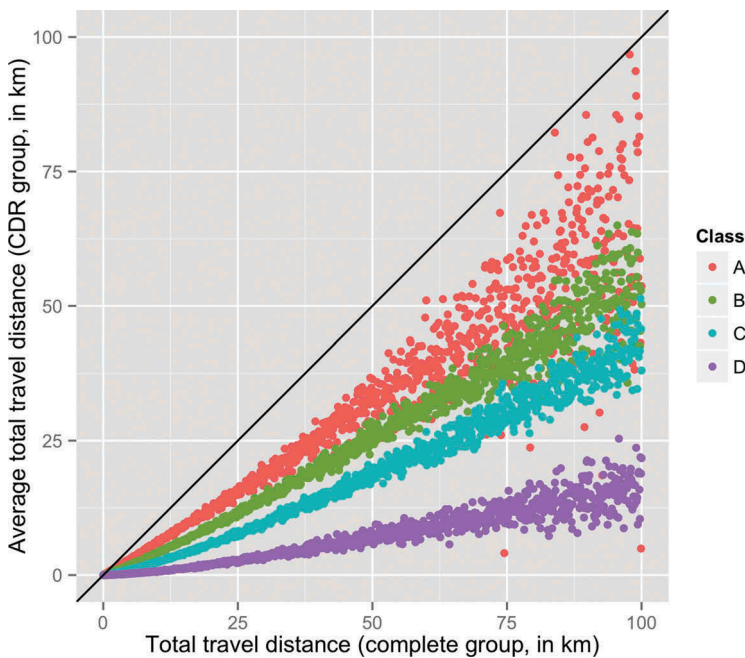
Figure 6. Total travel distance (complete group) vs. average total travel distance (CDR group).
