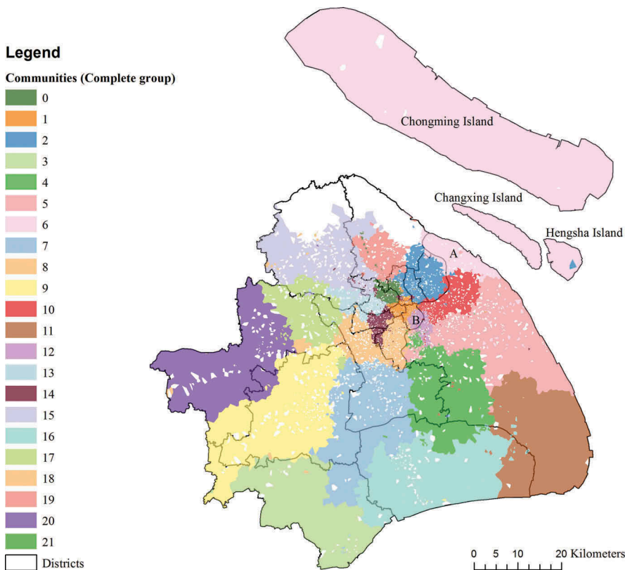
Figure 12. Detected communities based on the complete group.
