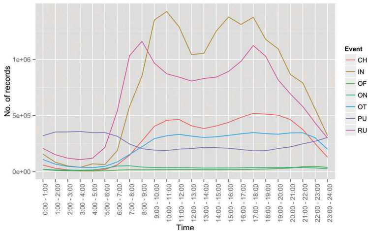
Figure 3. Temporal variation of the total number of each event.
