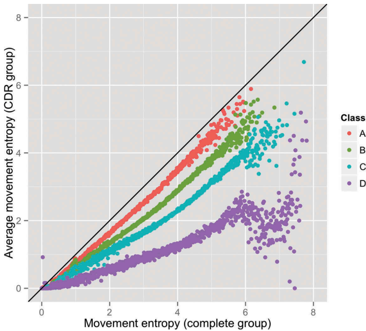
Figure 8. Movement entropy (complete group) vs. average movement entropy (CDR group).
