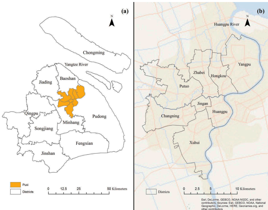
Figure 2. (a) Shanghai and its administrative districts. The orange areas represent the “Puxi” region, the downtown area of Shanghai. (b) Eight administrative districts in the “Puxi” region. “Puxi” and the Pudong districts are divided by the Huangpu River.
