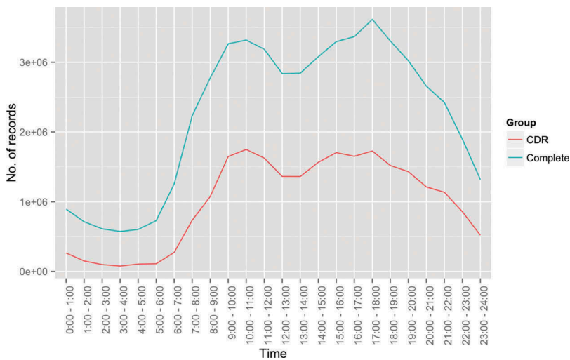
Figure 4. Temporal variation of the total number of records in the CDR group and the complete group.
