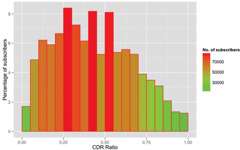
Figure 5. Distribution of subscribers under different ratio of CDRs.
