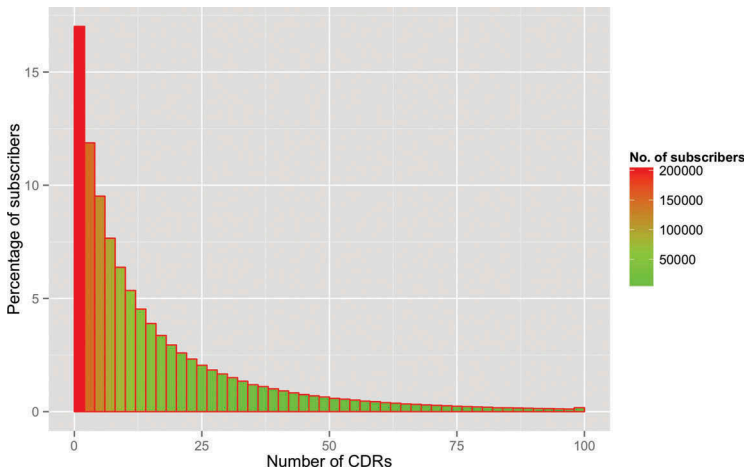
Figure 1. Distribution of subscribers under different intensity levels of phone communication.
